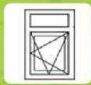
Tilt and turn window with fixed light above
